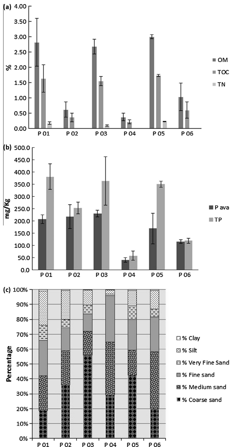
Fig. 2. Nutrients mean values and grain size fractions of intertidal zone sediments in Paraguaçu River estuary. (a) OM, TOC and TN in %; (b) P_{ava} and TP in \text{mg kg}^{-1} ; (c) grain size.
